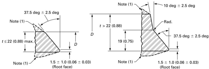
(a) Plain Bevel
