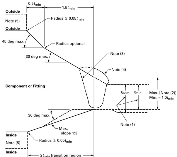
Figure 8-1 Maximum Envelope for Welding End Transitions
